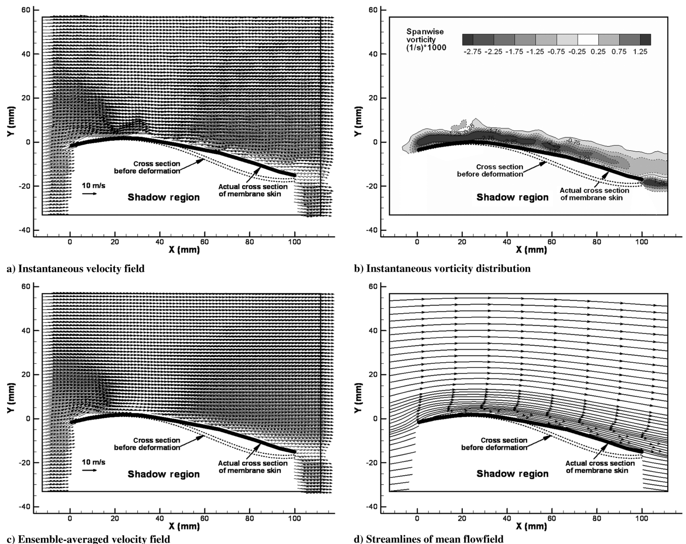
Fig. 8 PIV measurements in measurement plane 1 for the FM03 airfoil at \text{AOA} = 10.0^\circ .
